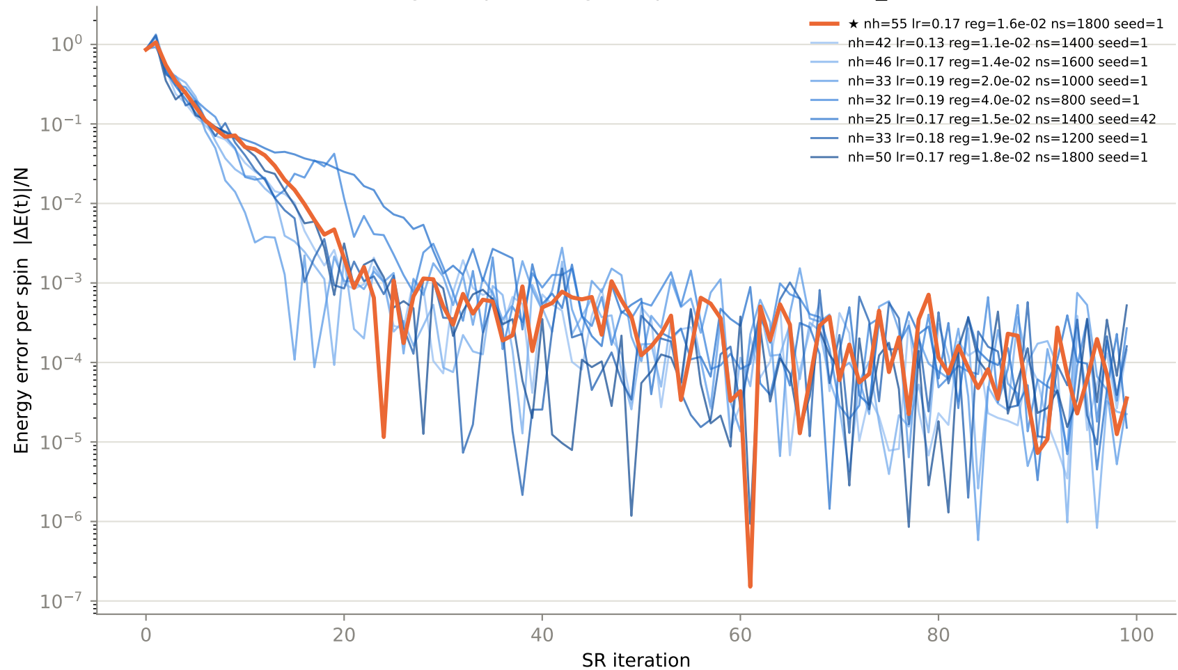
Convergence per config — top 8 of 92 trials, N16_J20.5
