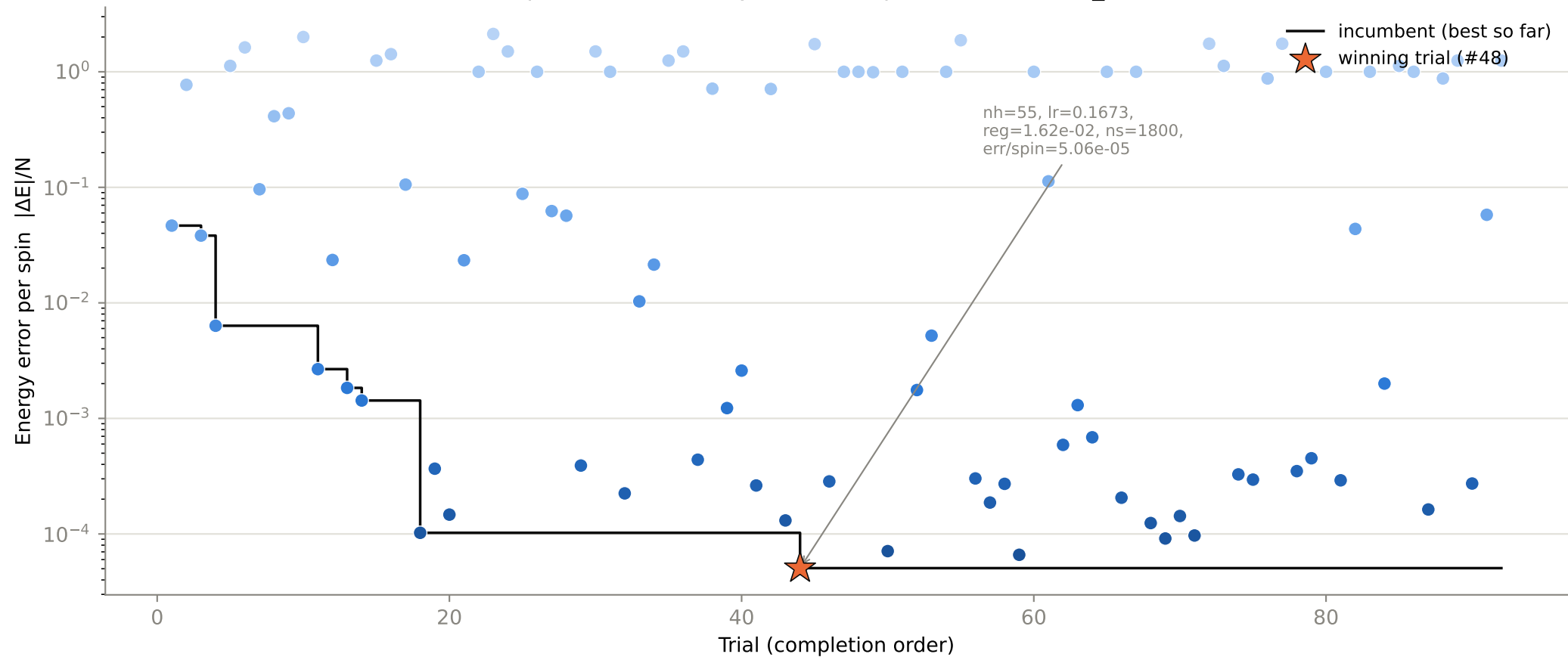
Optimization history — 92 completed trials, N16_J20.5
