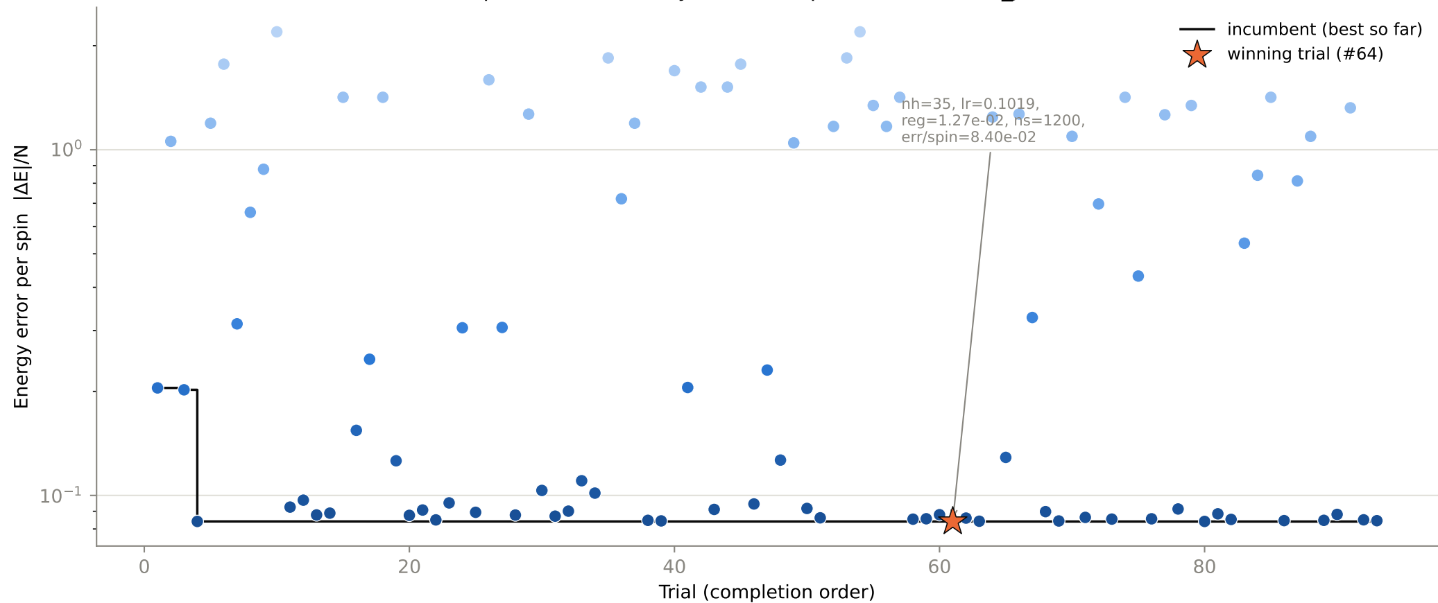
Optimization history — 93 completed trials, N16_J20.7
