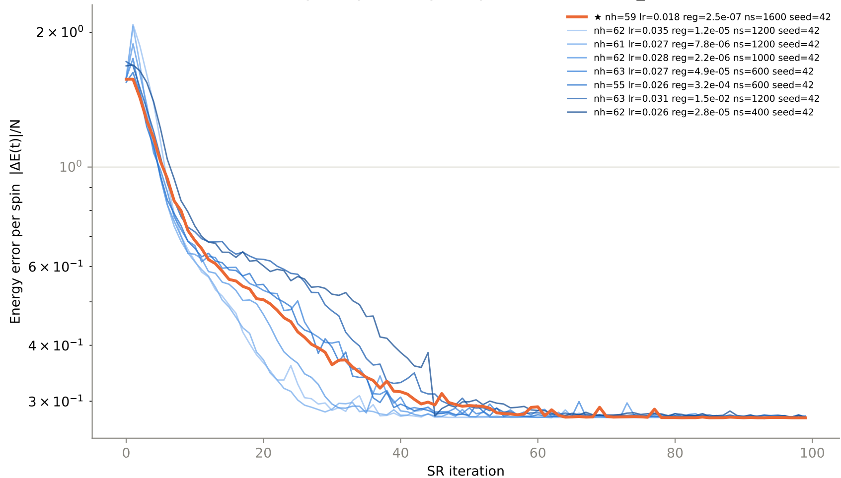
Convergence per config — top 8 of 85 trials, N16_J20.9
