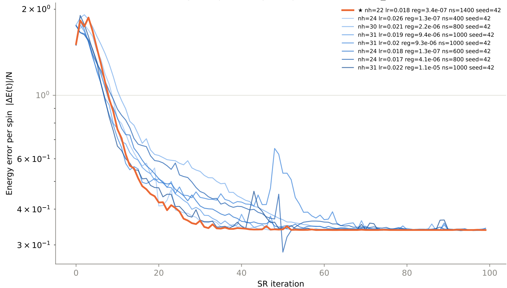
Convergence per config — top 8 of 79 trials, N8_J20.9
