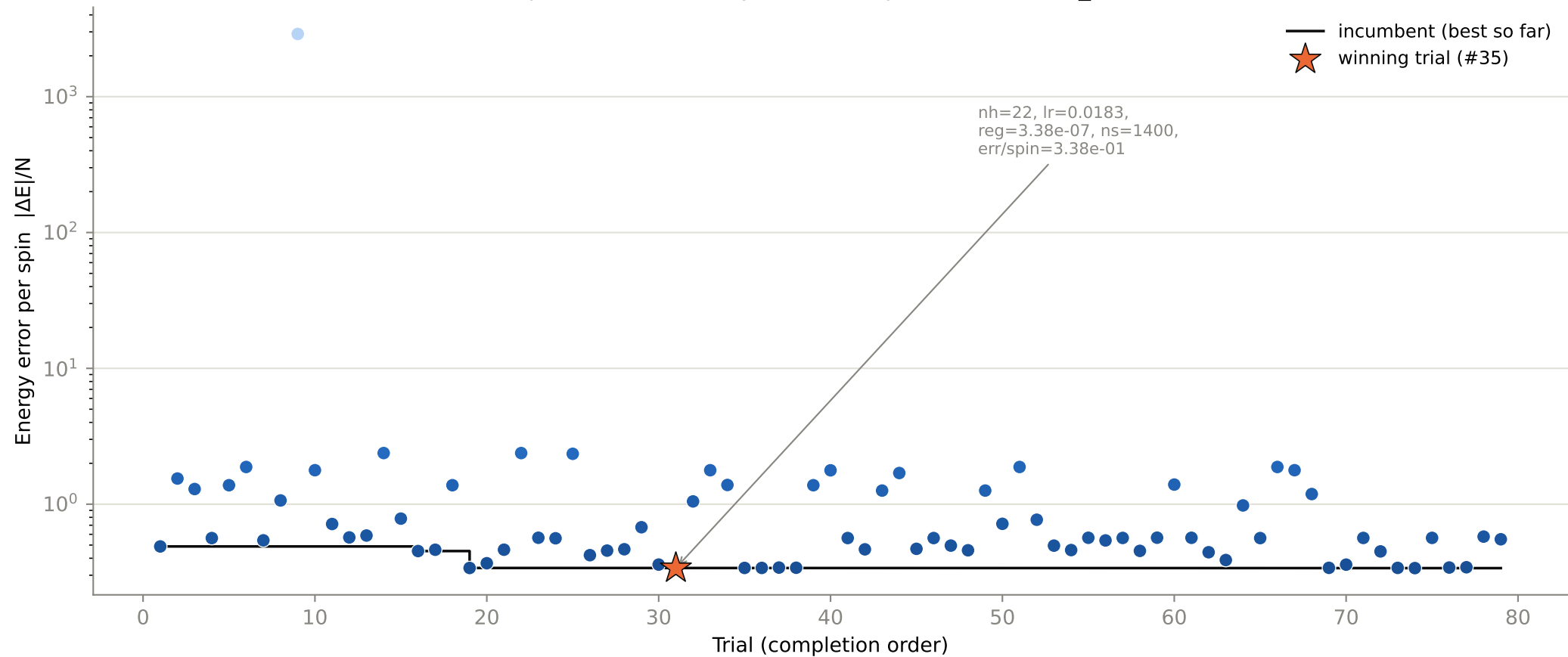
Optimization history — 79 completed trials, N8_J20.9
