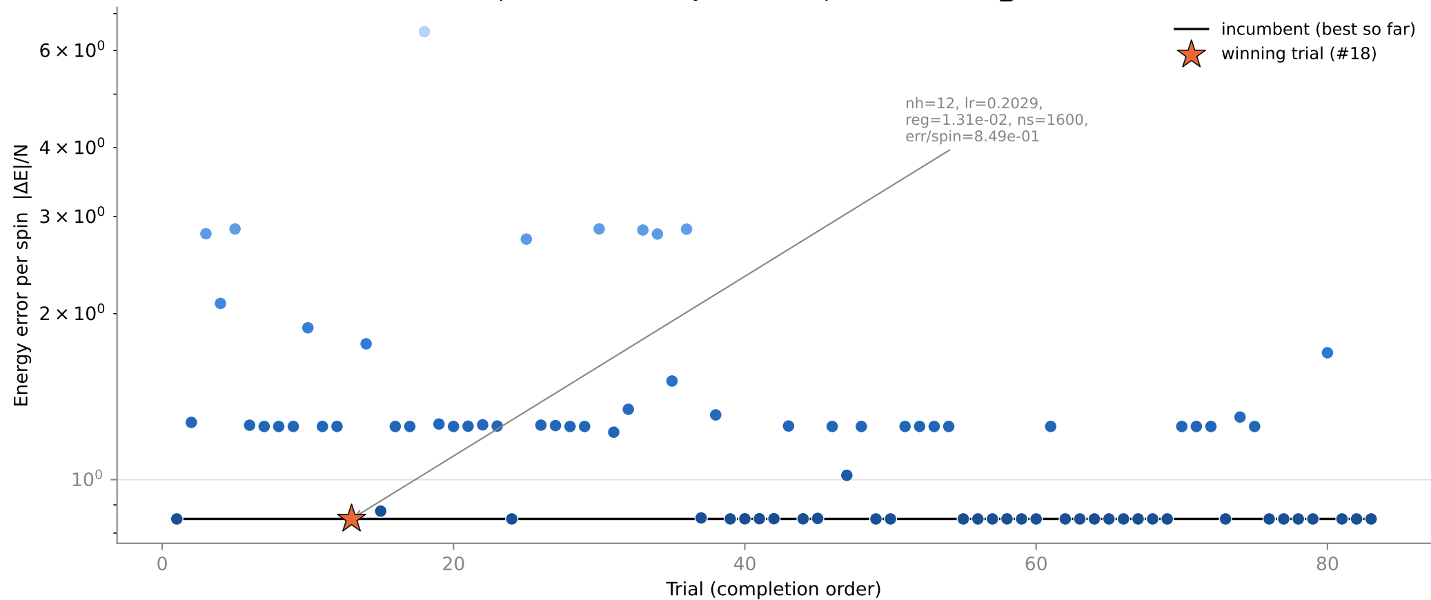
Optimization history — 83 completed trials, N8_J20.1
