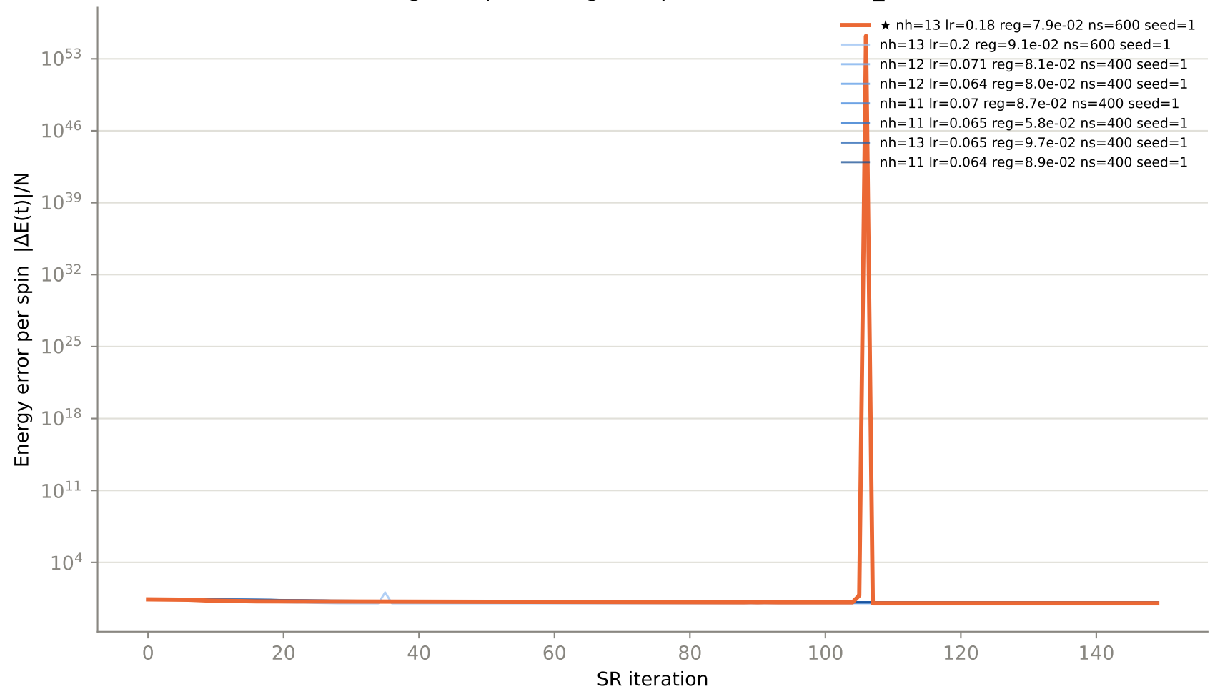
Convergence per config — top 8 of 60 trials, N8_delta0.5
