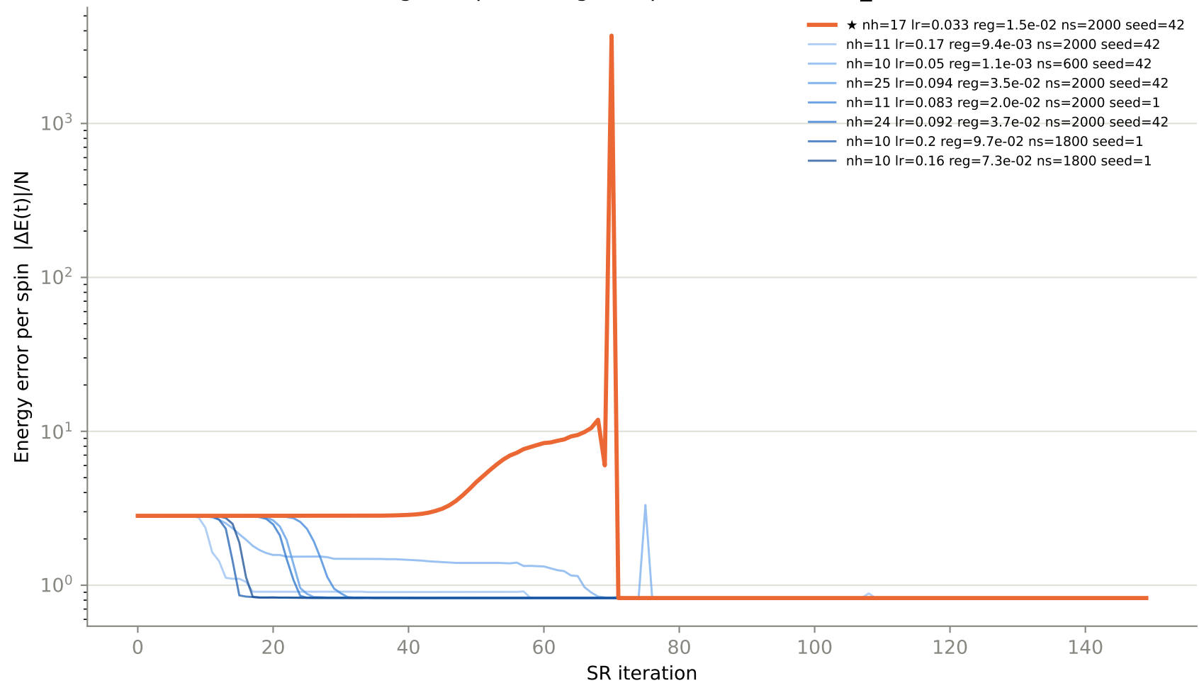
Convergence per config — top 8 of 29 trials, N8_delta1.0
