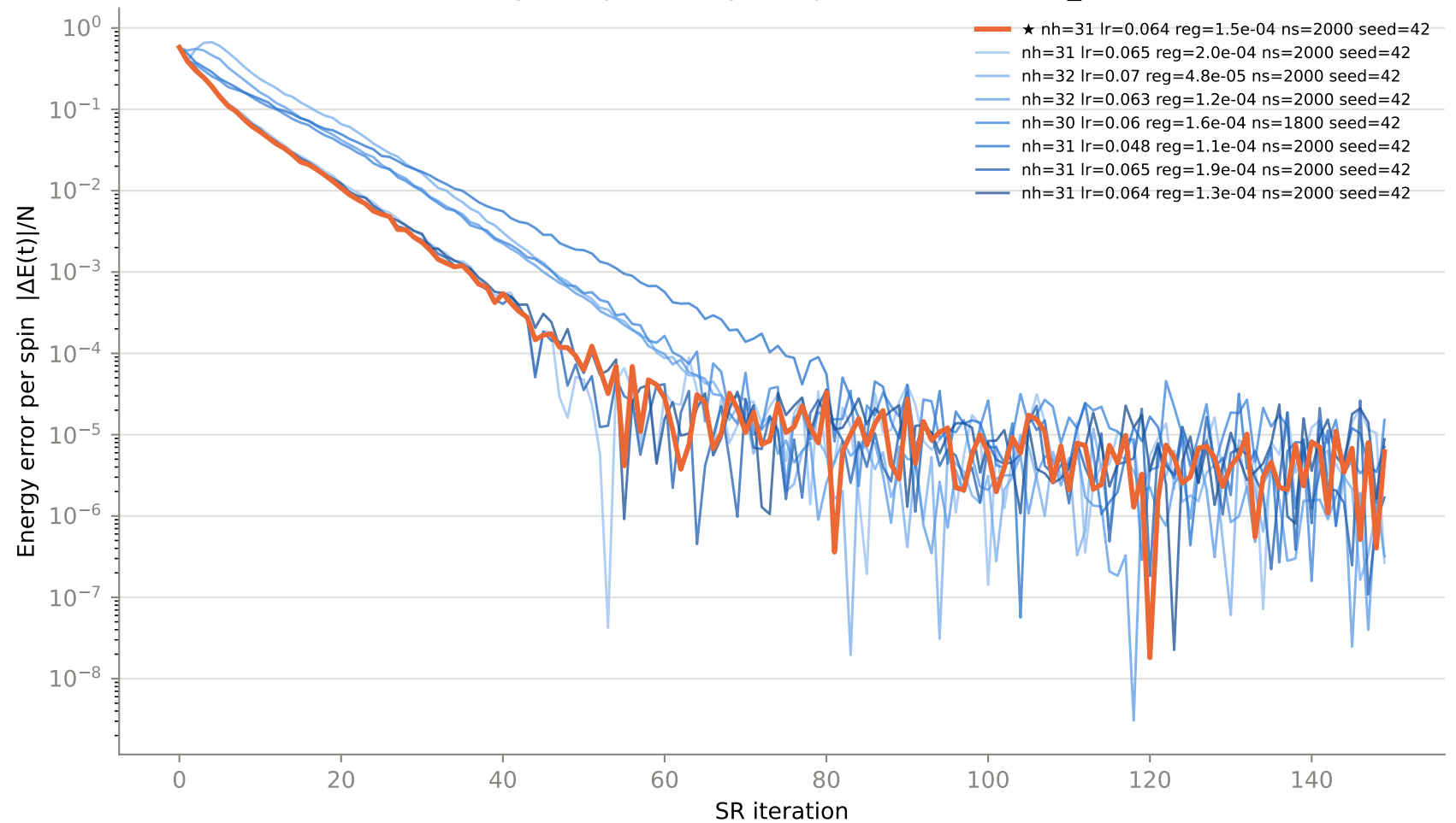
Convergence per config — top 8 of 90 trials, N8_J20.0
