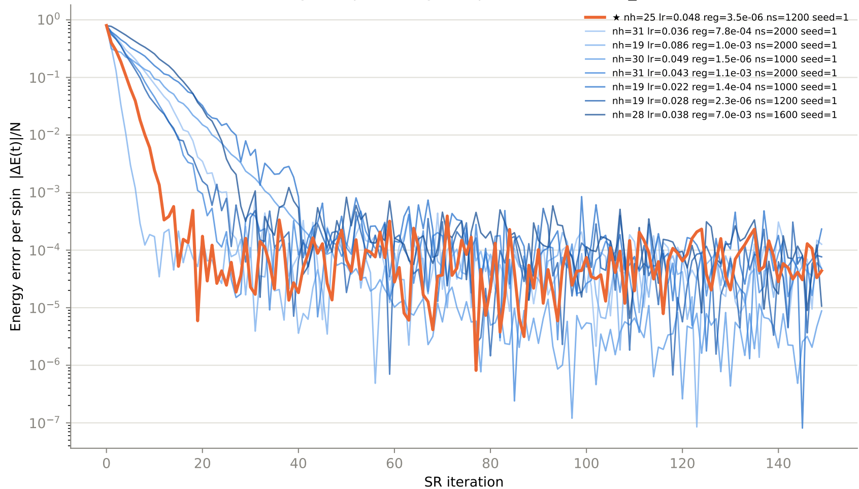
Convergence per config — top 8 of 86 trials, N8_J20.25
