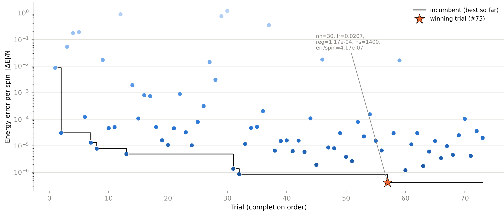
Optimization history — 73 completed trials, N8_J20.75
