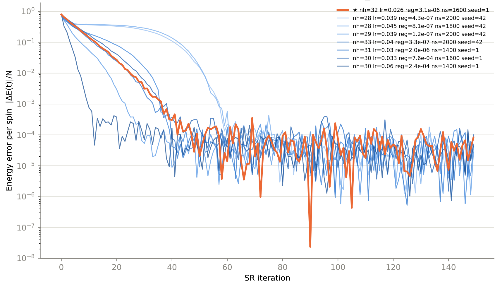
Convergence per config — top 8 of 82 trials, N12_J20.25
