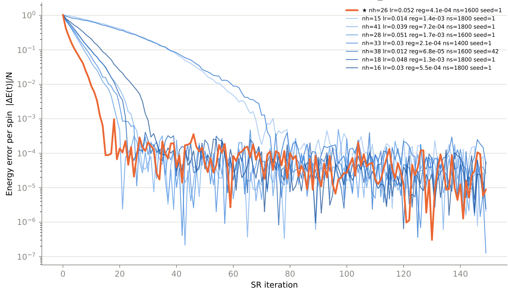
Convergence per config — top 8 of 91 trials, N12_J20.5
