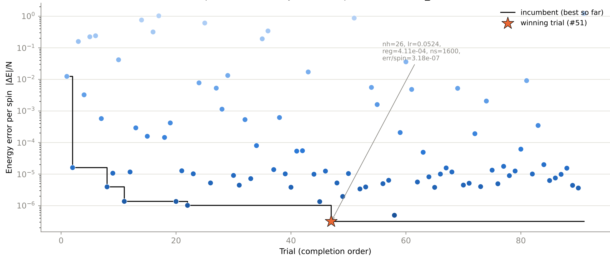
Optimization history — 91 completed trials, N12_J20.5
