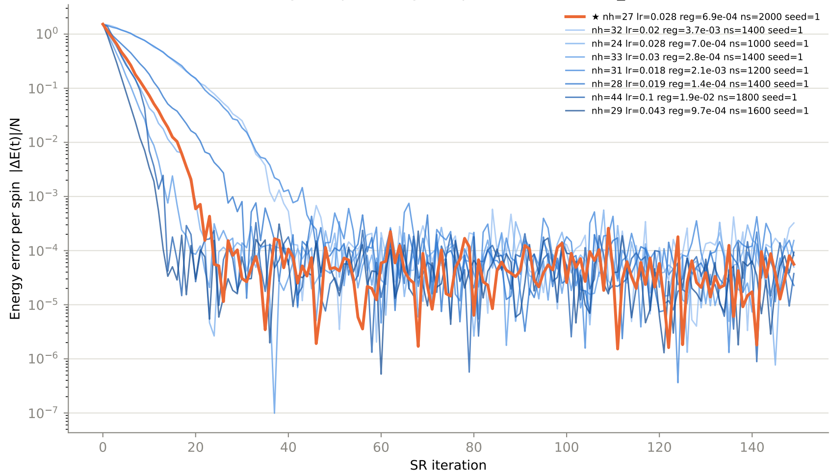
Convergence per config — top 8 of 85 trials, N12_J21.0
