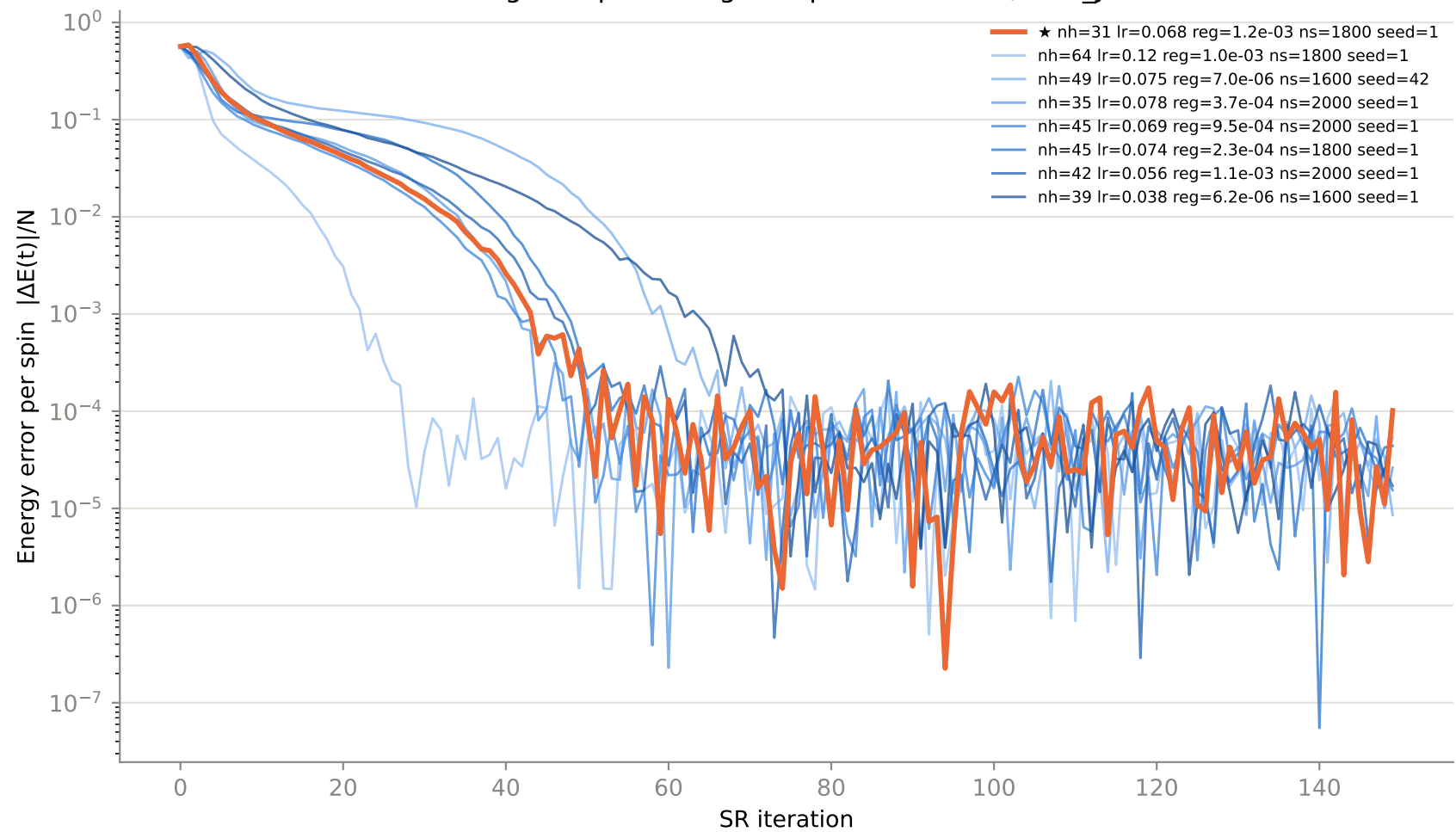
Convergence per config — top 8 of 78 trials, N16_J20.0
