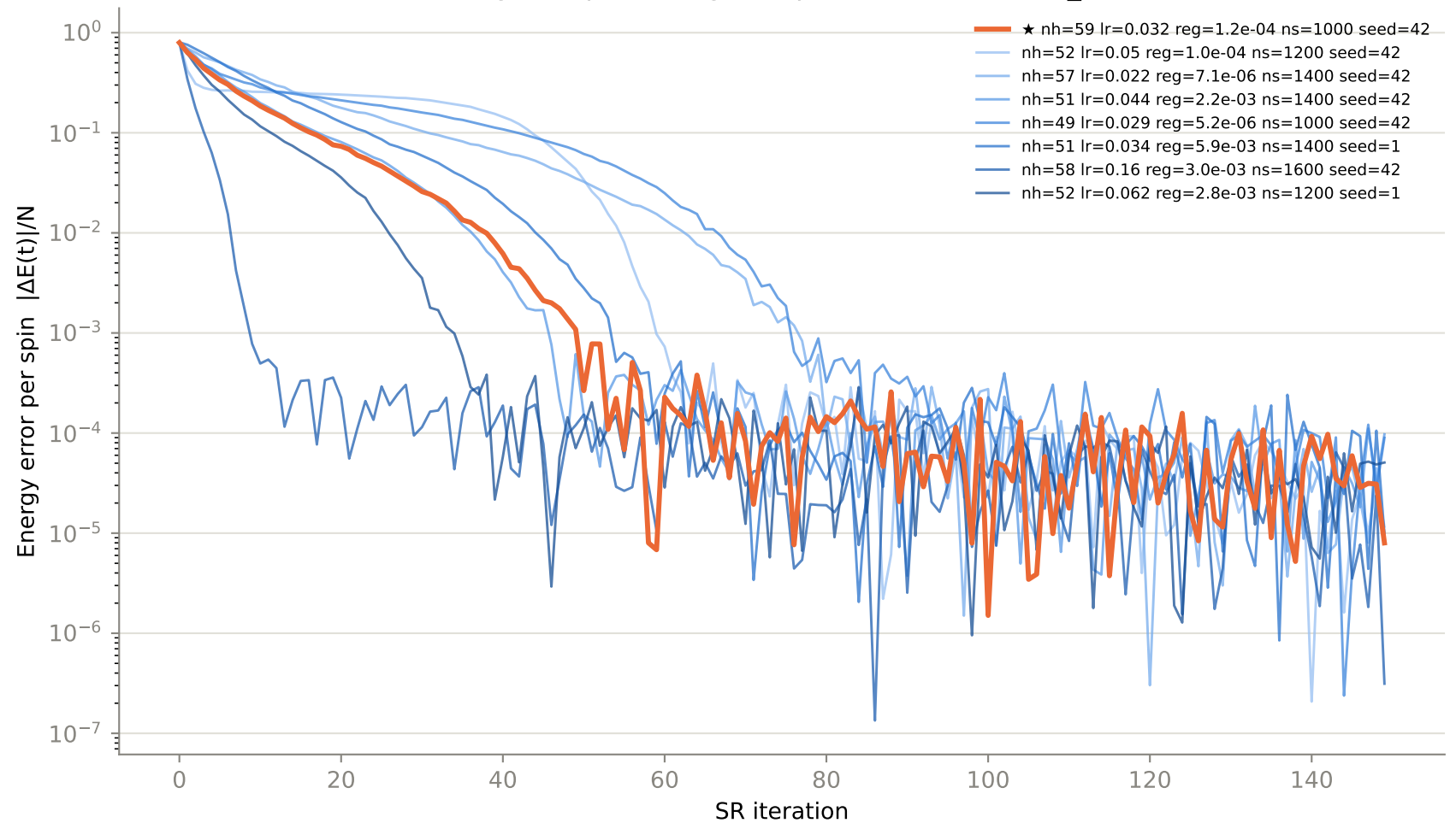
Convergence per config — top 8 of 83 trials, N16_J20.25
