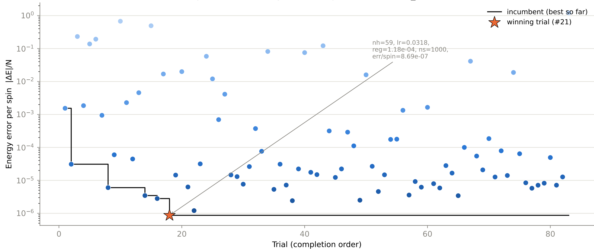
Optimization history — 83 completed trials, N16_J20.25
