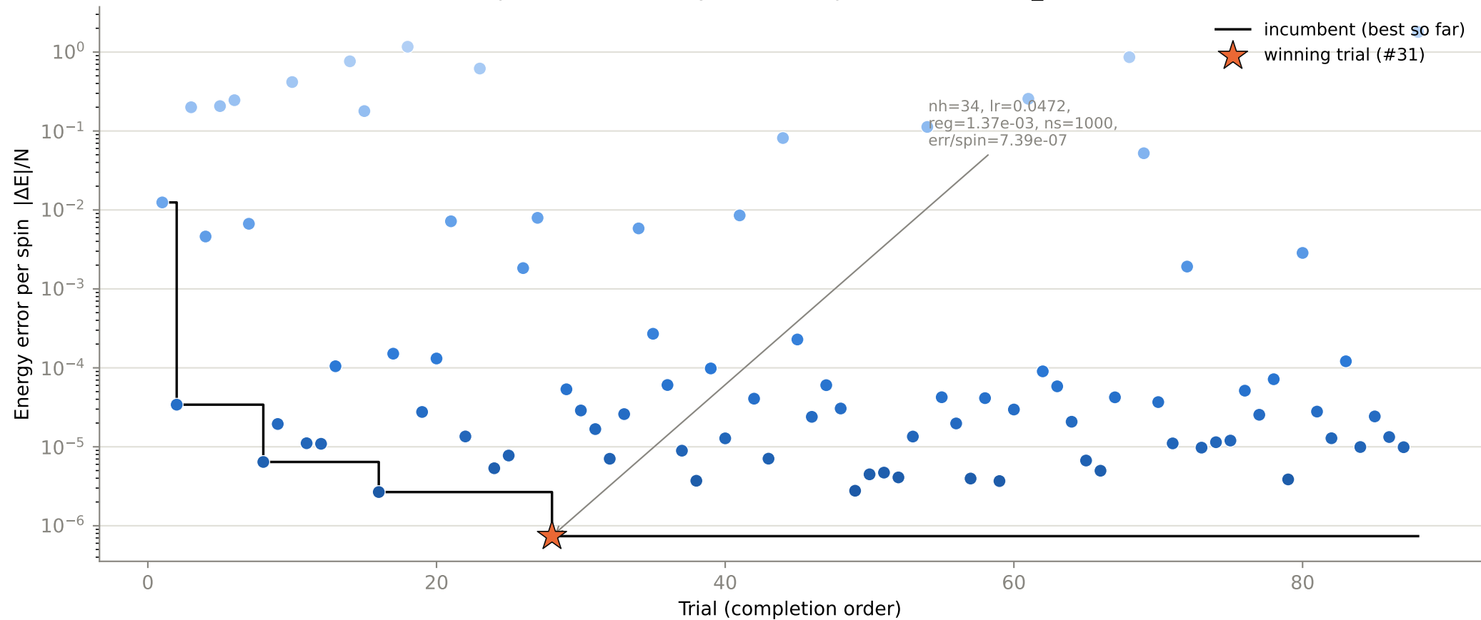
Optimization history — 88 completed trials, N16_J20.5
