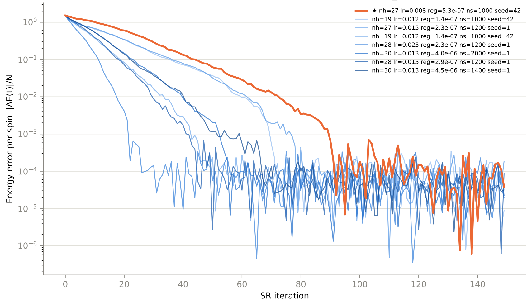
Convergence per config — top 8 of 88 trials, N16_J21.0
