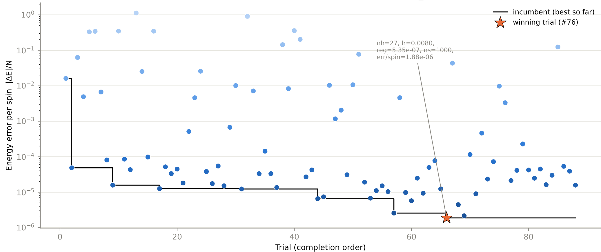
Optimization history — 88 completed trials, N16_J21.0
