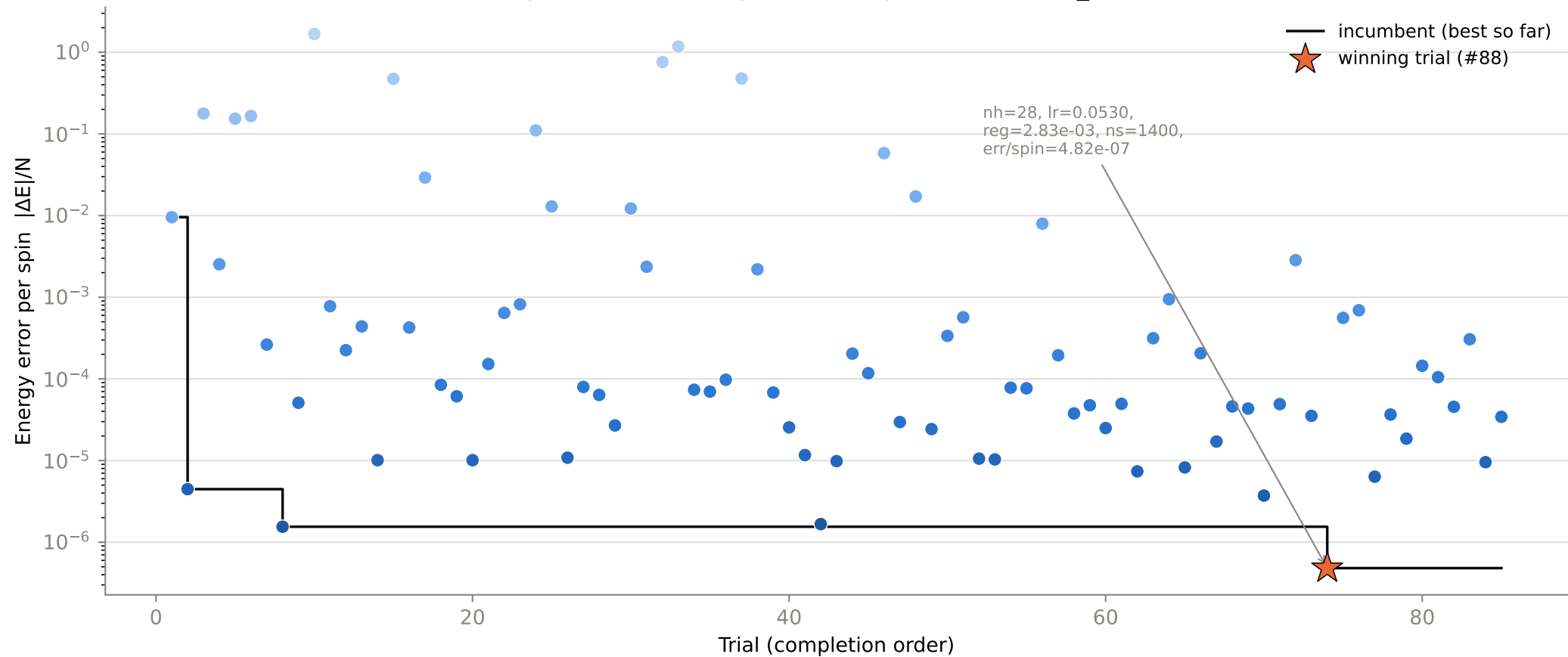
Optimization history — 85 completed trials, N8_J20.25
