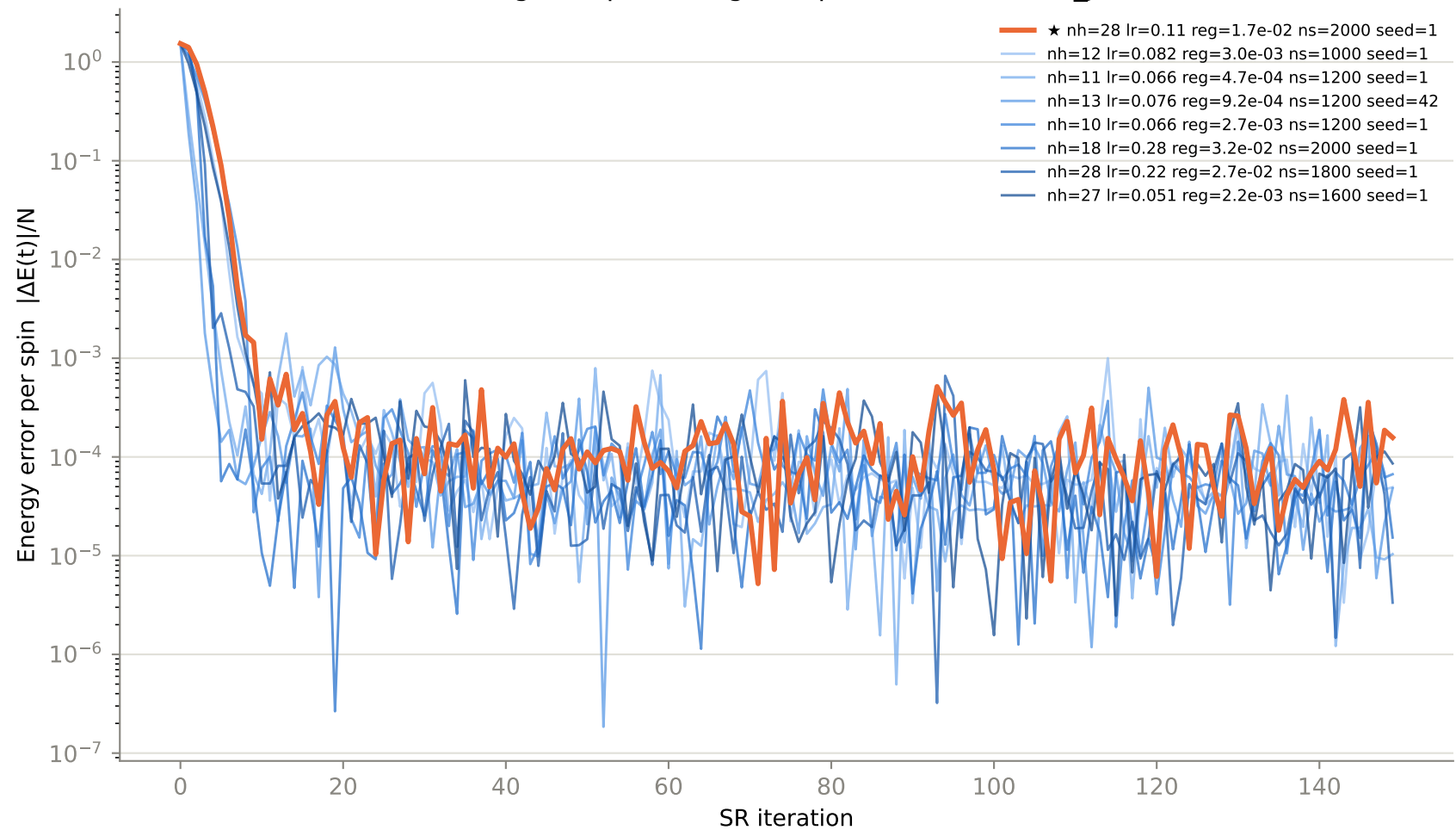
Convergence per config — top 8 of 77 trials, N8_J21.0
