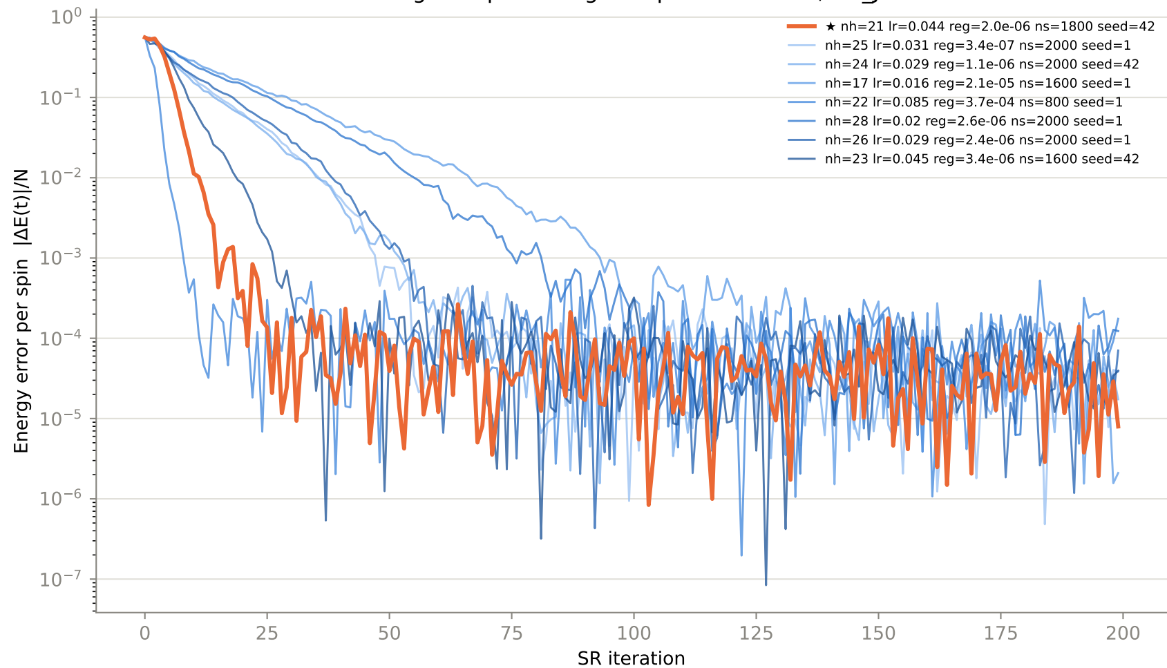
Convergence per config — top 8 of 77 trials, N8_J20.0
