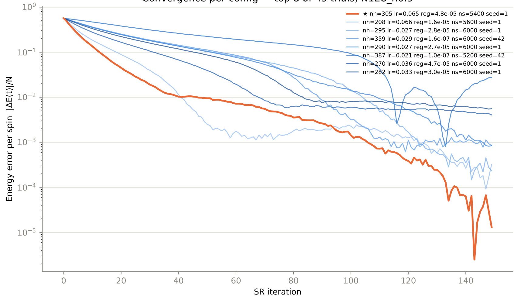
Convergence per config — top 8 of 45 trials, N128_h0.5
