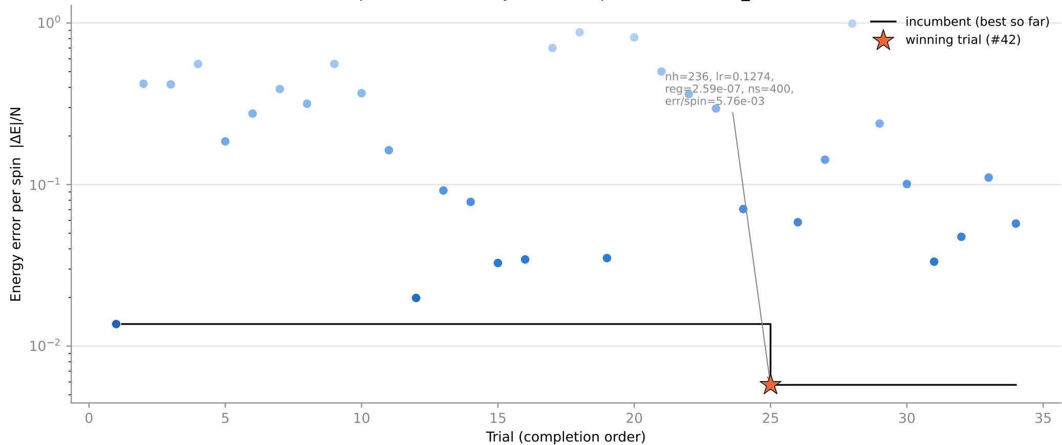
Optimization history — 34 completed trials, N64_h0.5
