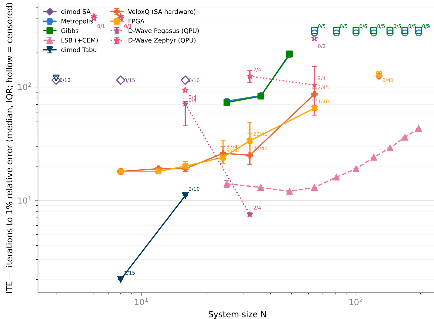
(A) Iterations-to-epsilon vs. N
