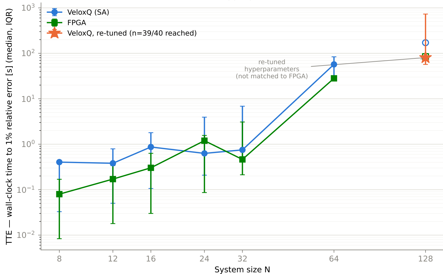
Time-to-epsilon vs. system size TFIM 1D, h=0.5 , matched hyperparameters, VeloxQ vs. FPGA
