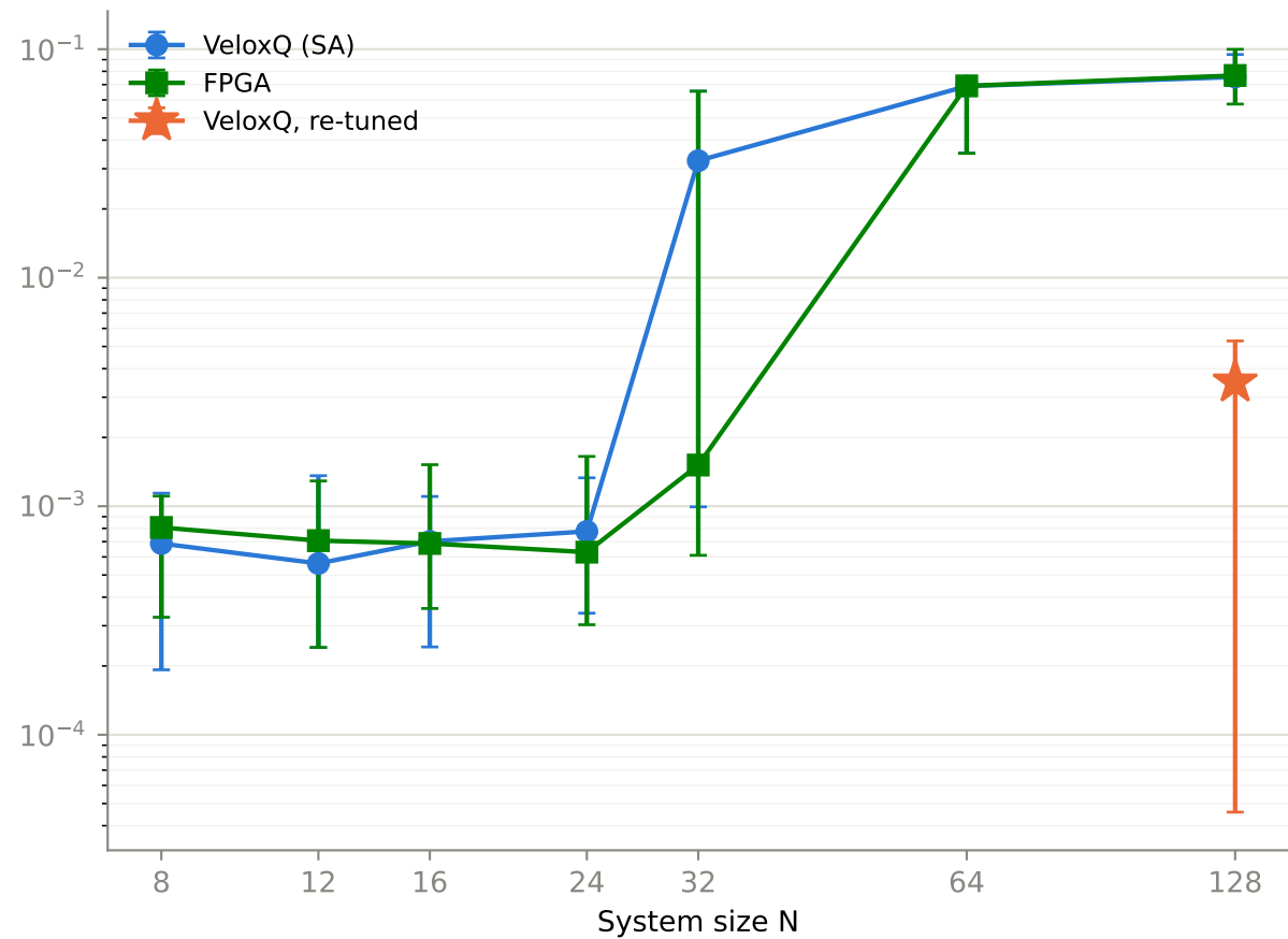
(B) TFIM, h=0.5 , 100 iterations
