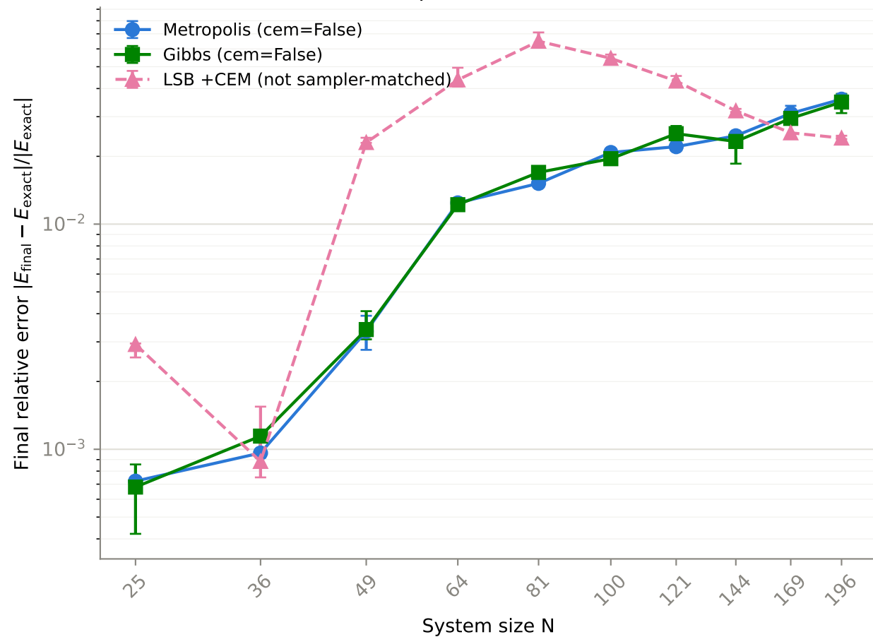
(A) TFIM critical point ( h=1.0 ), 300 iterations
