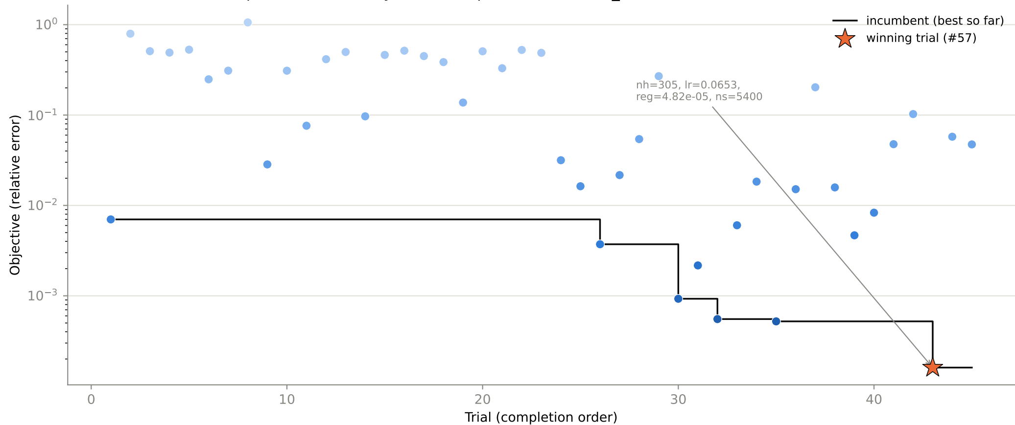
Optimization history — 45 completed trials, tfim_1d N=128, h=0.5, VeloxQ-SA
