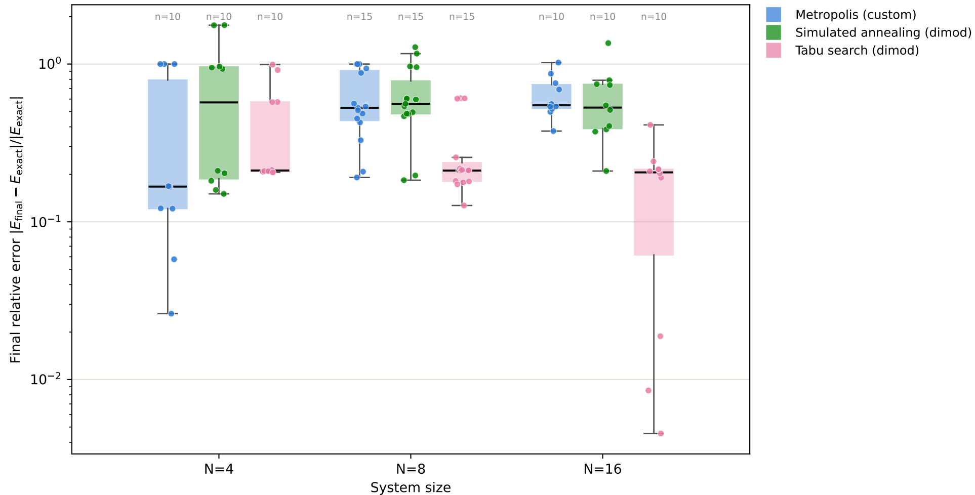
Solver comparison at fixed hyperparameters, TFIM critical point ( h=1.0 ) 100 SR iterations, all available seeds per cell (no best-of)
