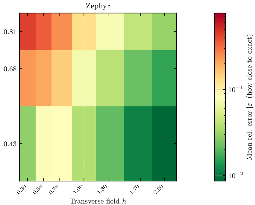
N = 16 — accuracy vs. (sparsity, h )
