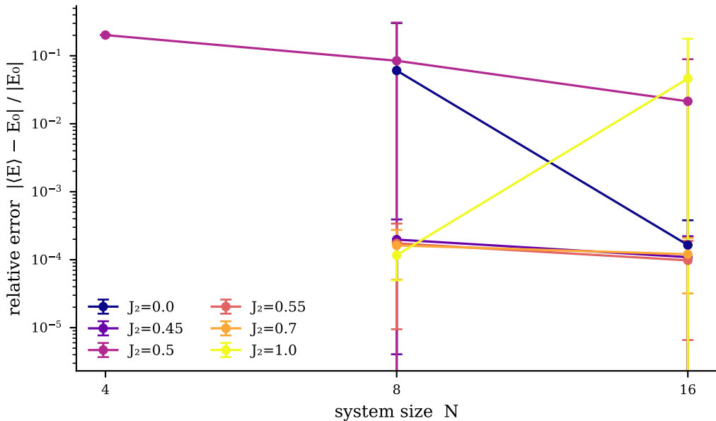
Energy error scaling with system size (metropolis, tail-mean \pm std over seeds)
