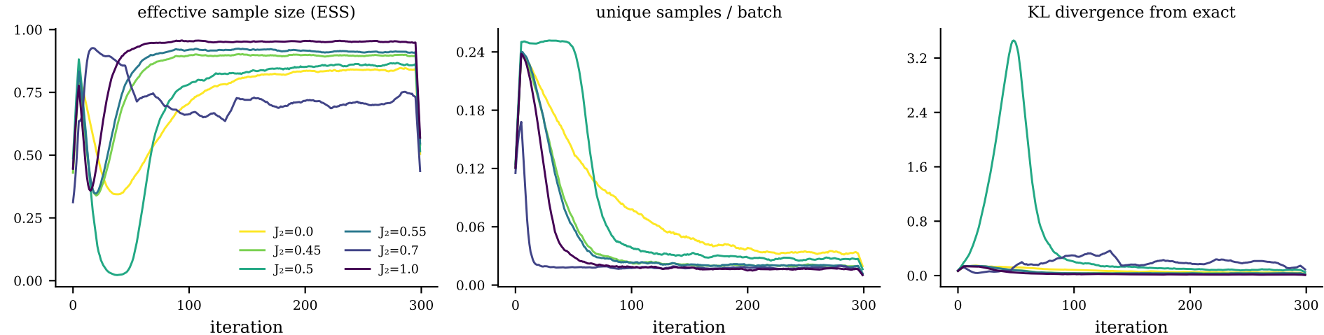
Sample quality over training — J1-J2 Ising N=8, metropolis (seed 1)
