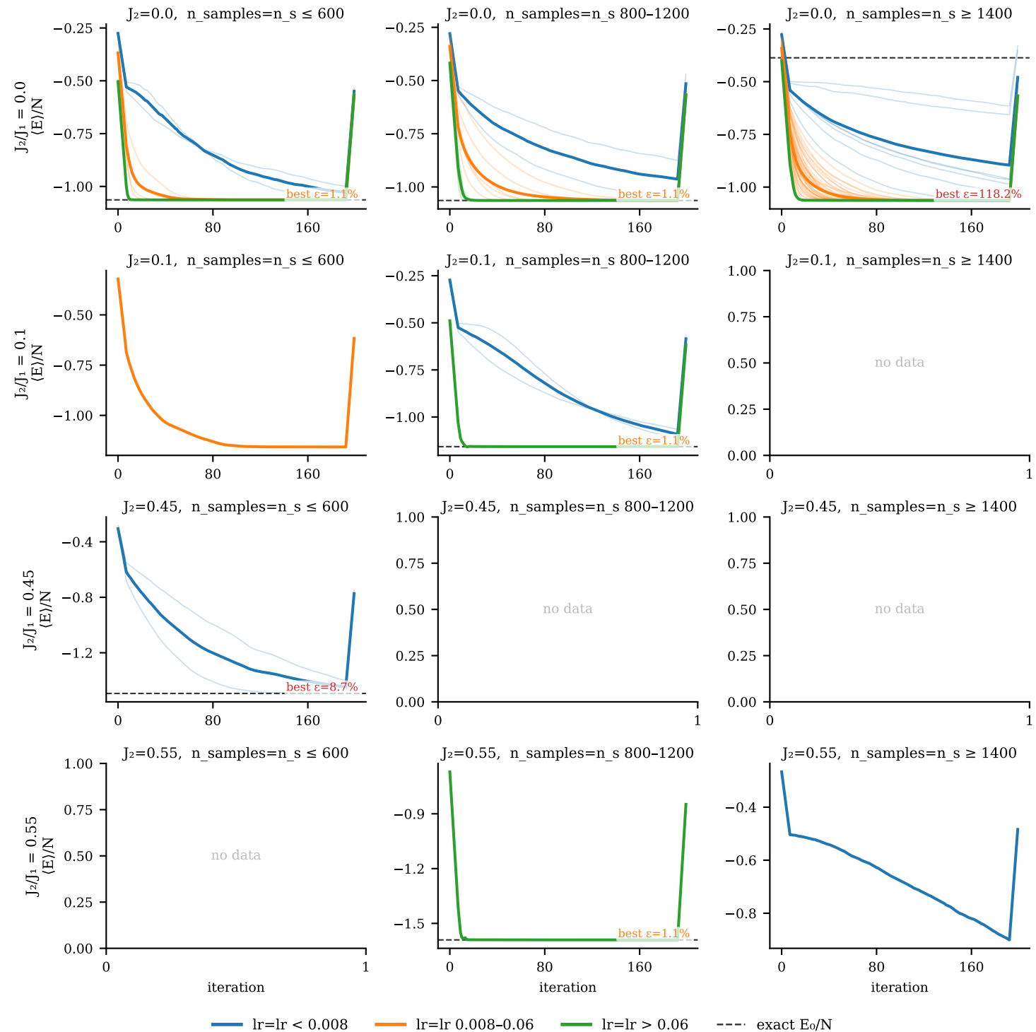
Gibbs sampler — J1-J2 Ising chain (Optuna-searched hyperparams) Rows: frustration J_2/J_1 · Cols: batch size n_{\text{samples}} · Colour: learning rate range
