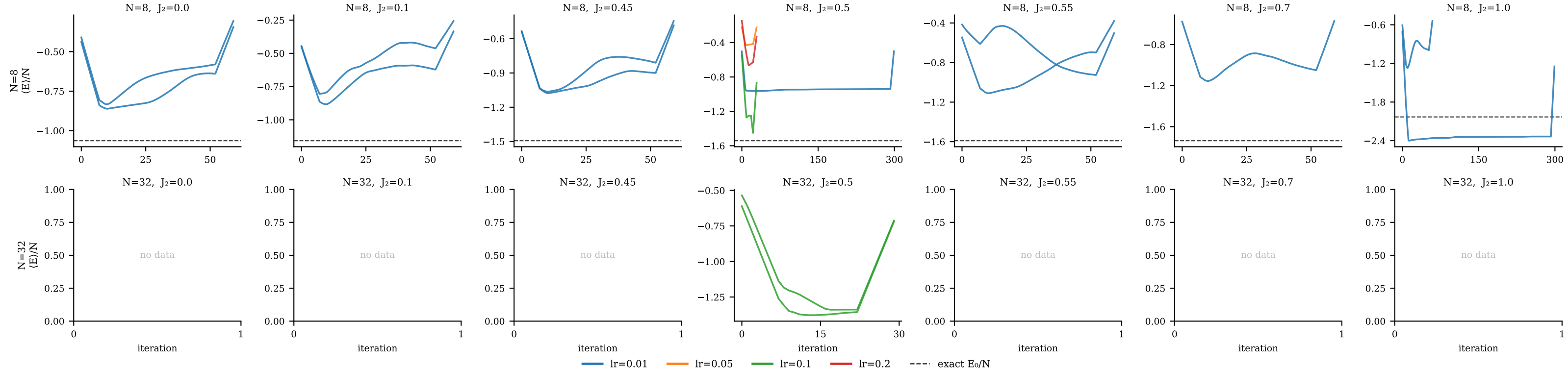
D-Wave Zephyr QPU — J1-J2 Ising chain Rows: system size N · Cols: frustration J_2/J_1 · Colour: learning rate
