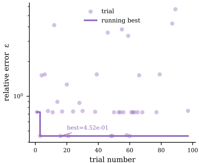
lsb (39 trials)
