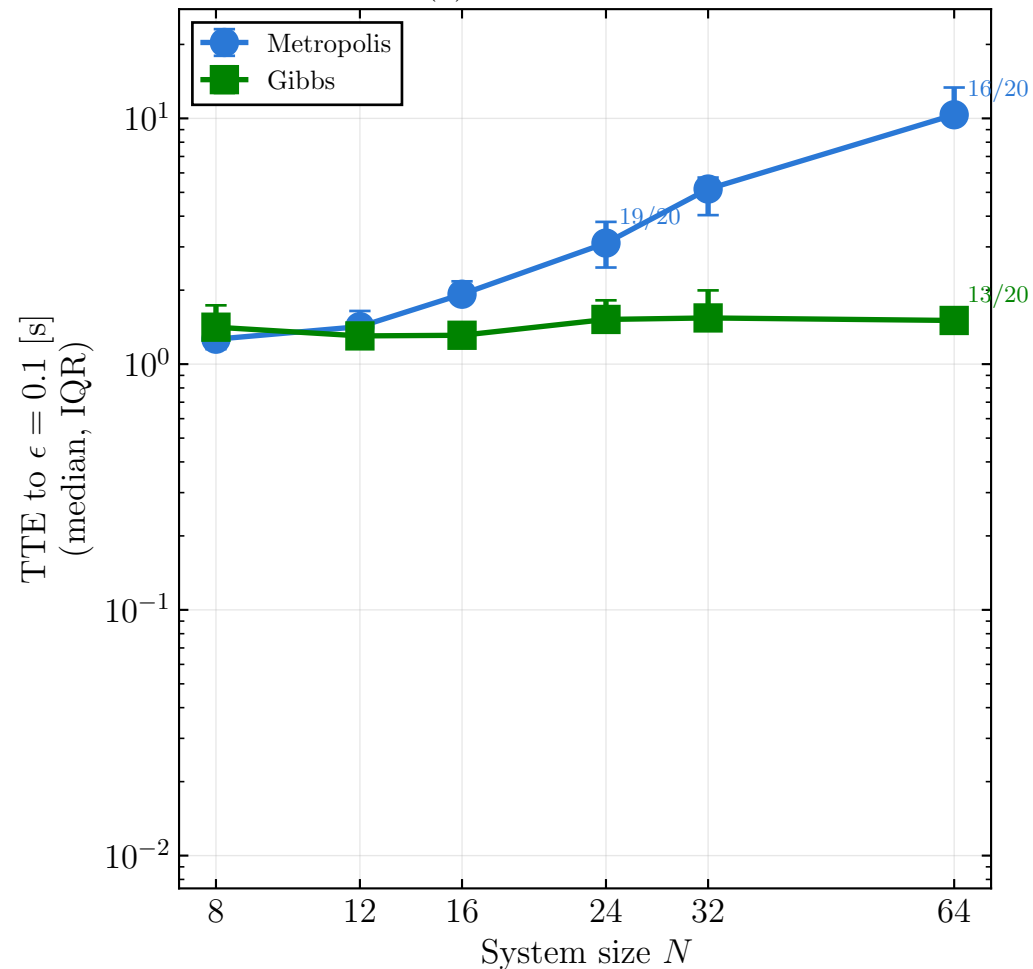
(a) Classical samplers
