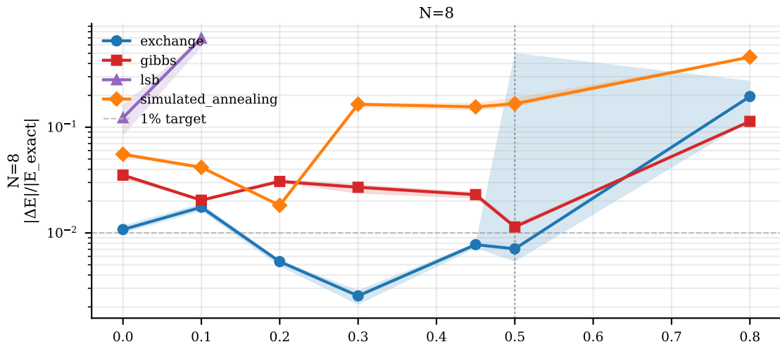
Relative energy error at convergence vs J_2 (heisenberg J1-J2) |\Delta E|/|E_{\text{exact}}| , rolling std < 1.0% \cdot|E_{\text{exact}}| , window=20
