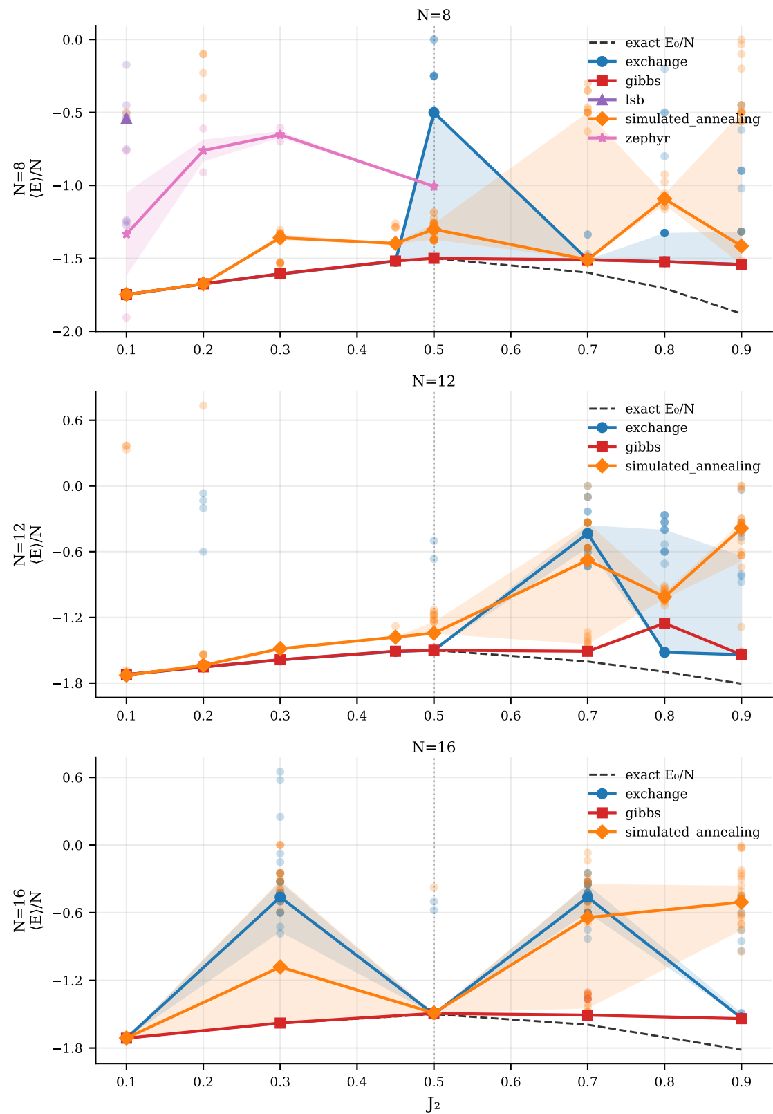
Converged \langle E \rangle / N per spin vs J_2 (heisenberg_j1j2_1d (isotropic Heisenberg)) Median \pm IQR over seeds
