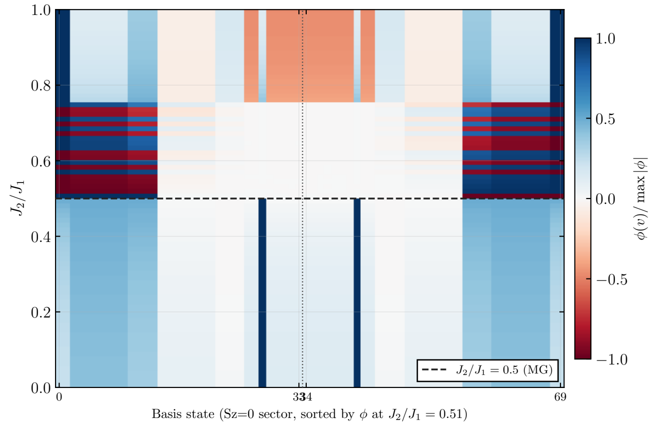
Sign structure heatmap — N = 8 , S_z = 0 sector (70 states)
