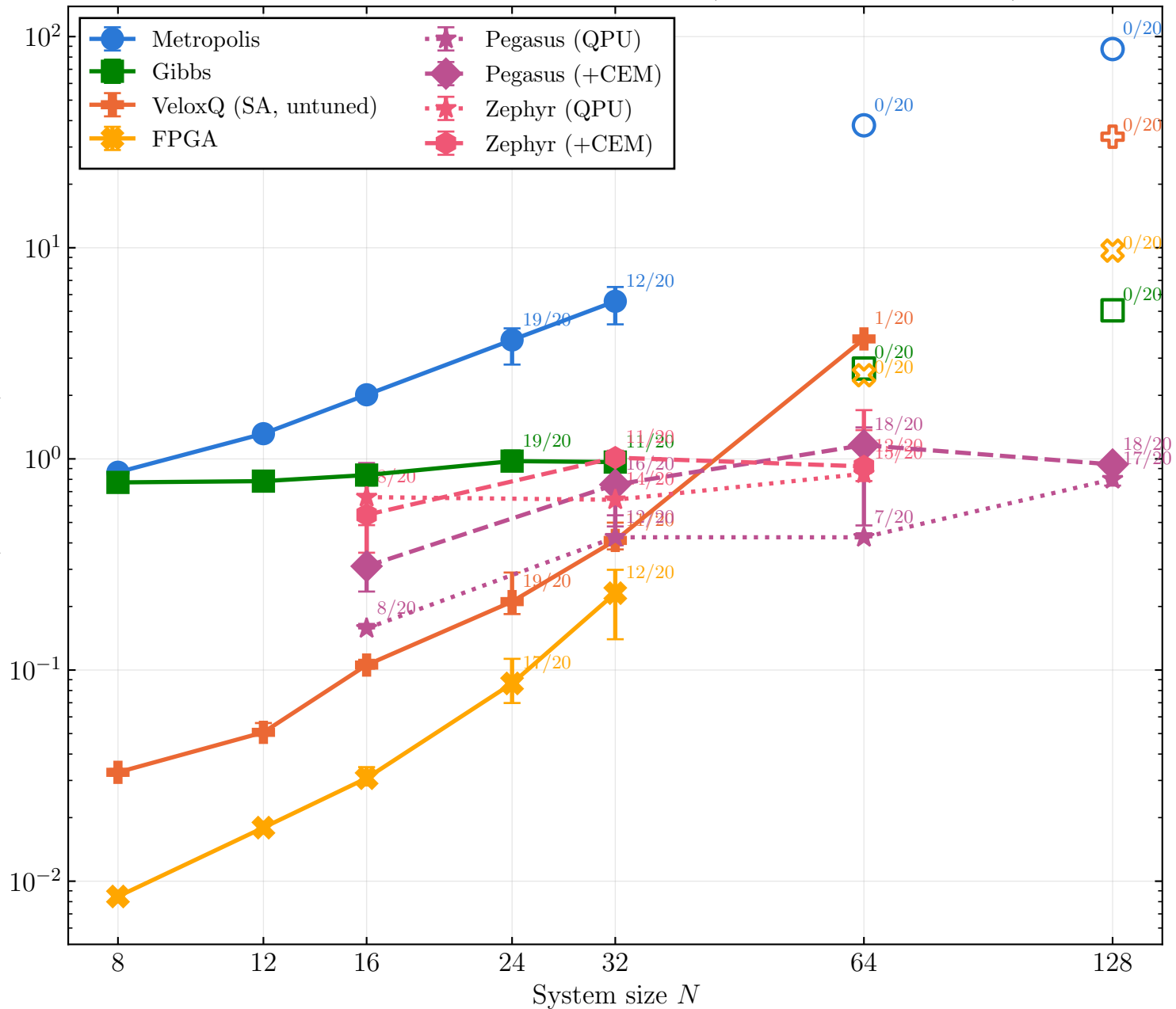
Time-to- \epsilon vs. system size N — all solvers (hyperparameter-matched)
