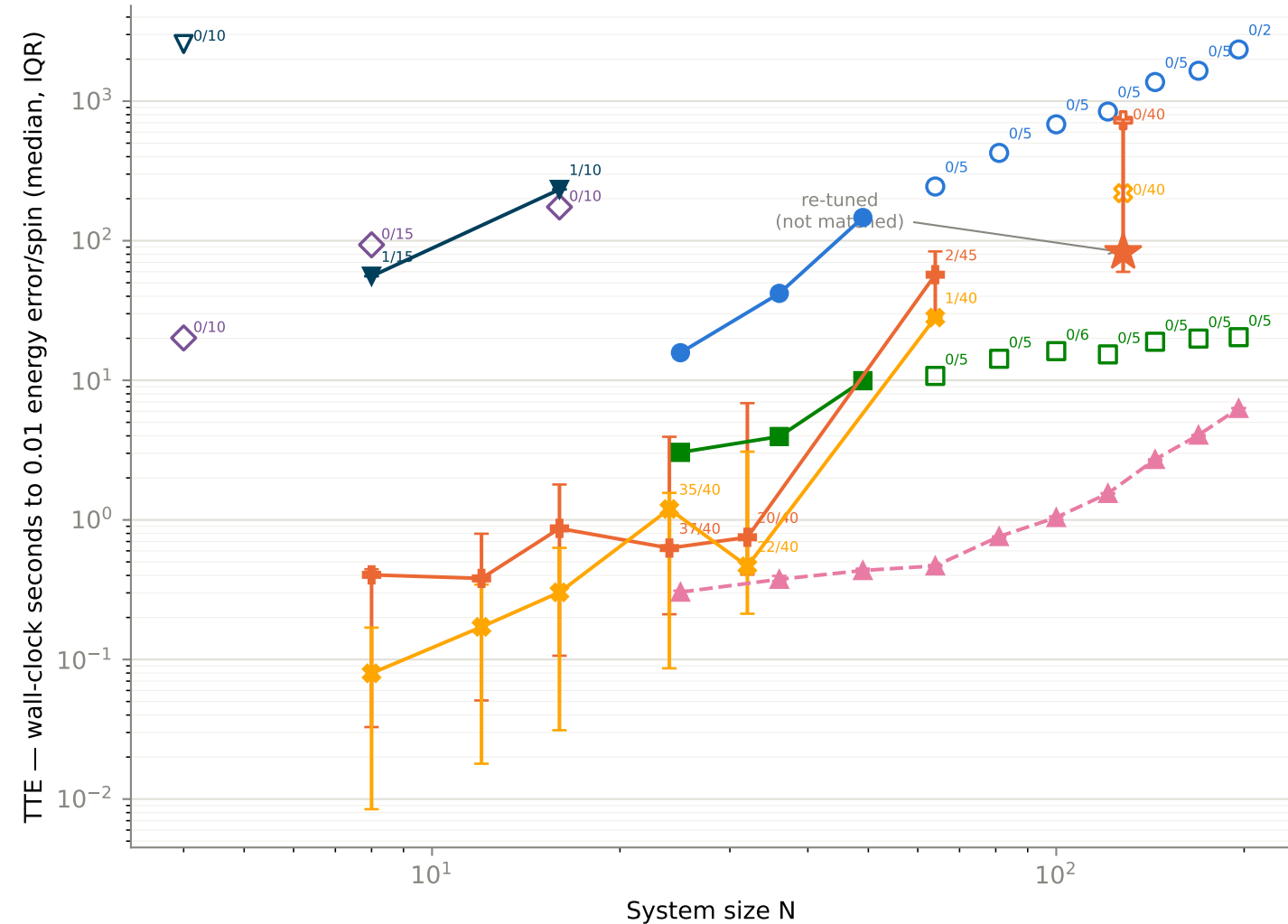
(B) Time-to-epsilon vs. N (D-Wave QPU omitted, no timing recorded)
