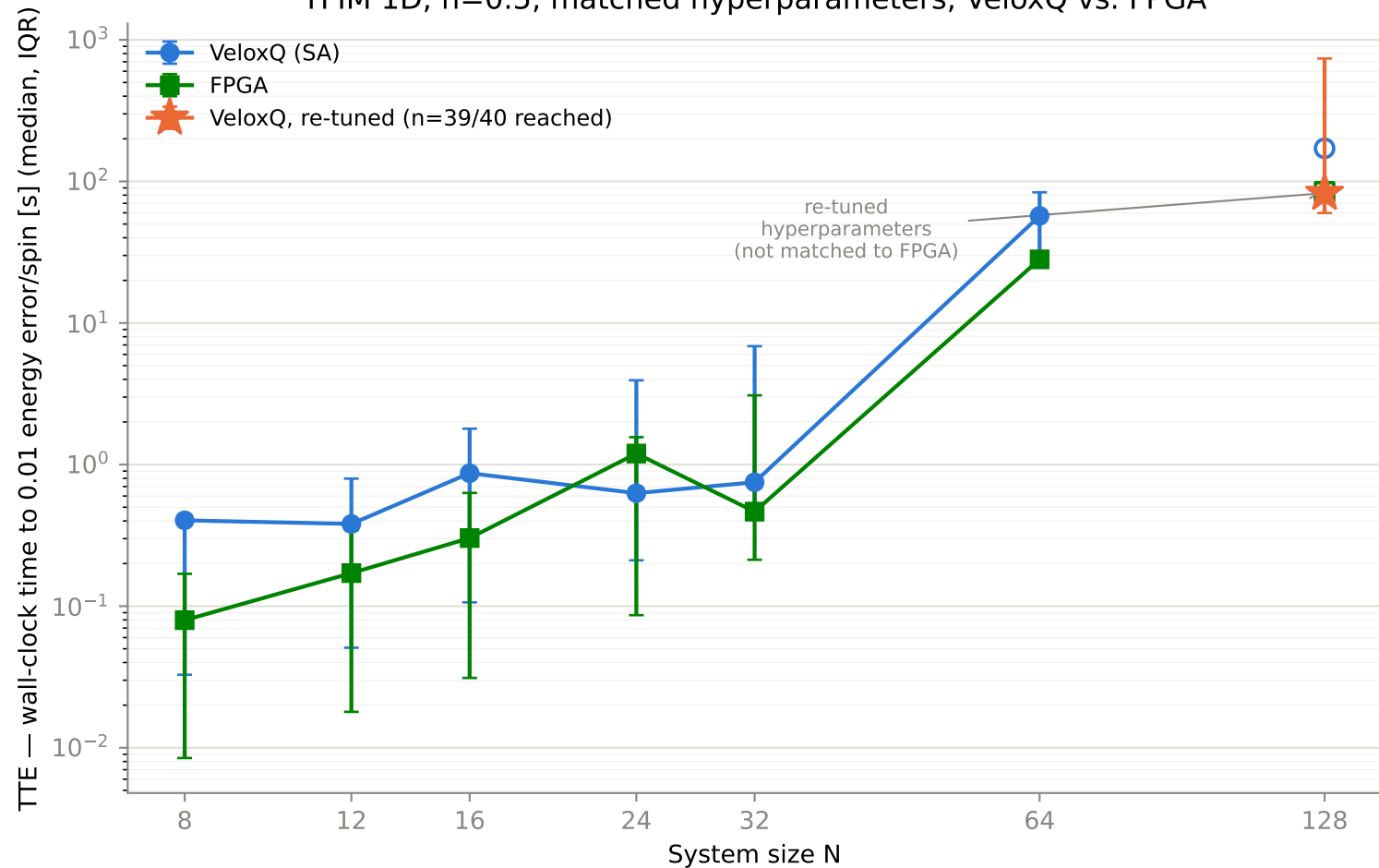
Time-to-epsilon vs. system size TFIM 1D, h=0.5 , matched hyperparameters, VeloxQ vs. FPGA
