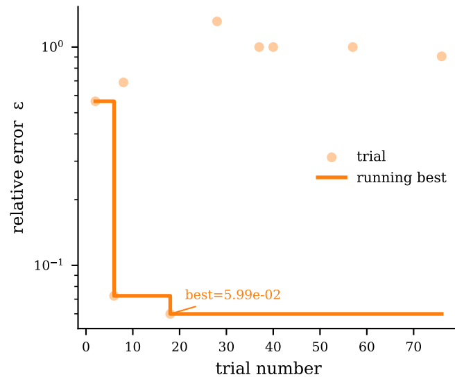
simulated_annealing (9 trials)
