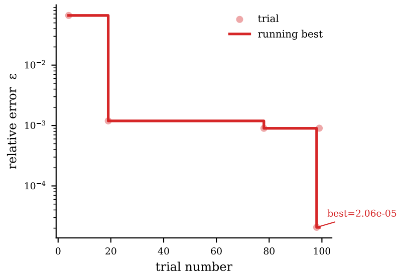
gibbs (5 trials)
