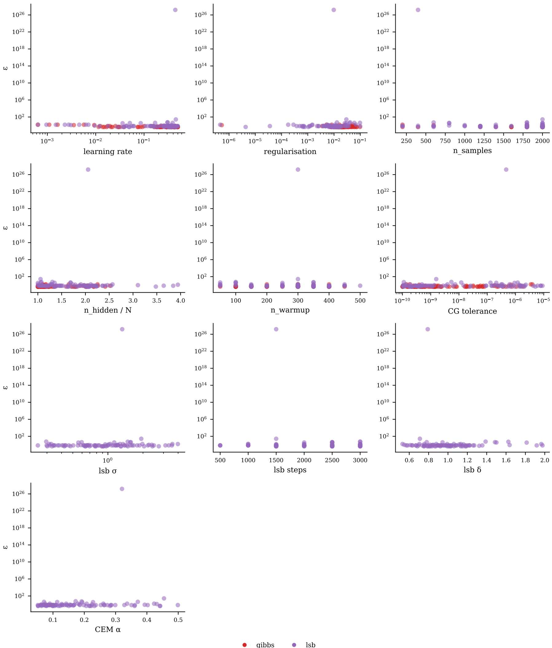
Hyperparameter sensitivity — heisenberg_j1j2_1d/j1j2_gibbs_lsb_v1/N8_J20.0
