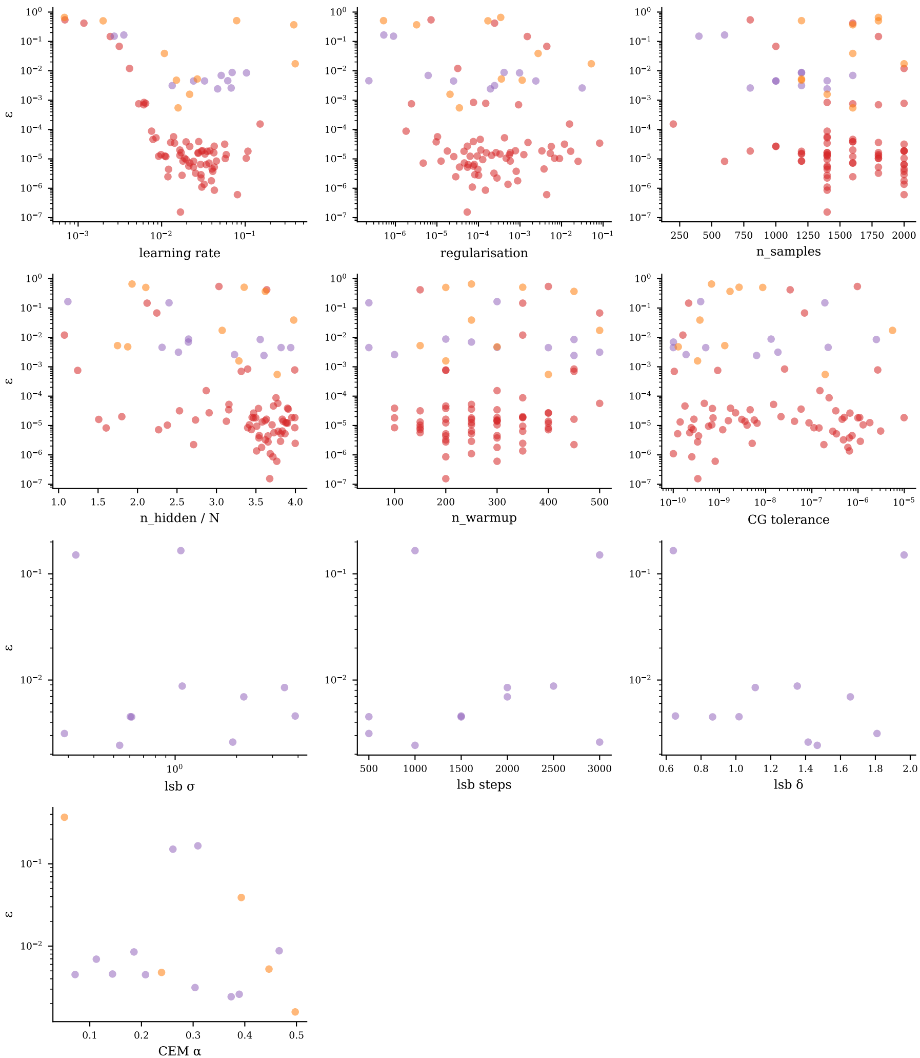
Hyperparameter sensitivity — j1j2_1d/j1j2_1d_20260527_170753/N16_J20.75
