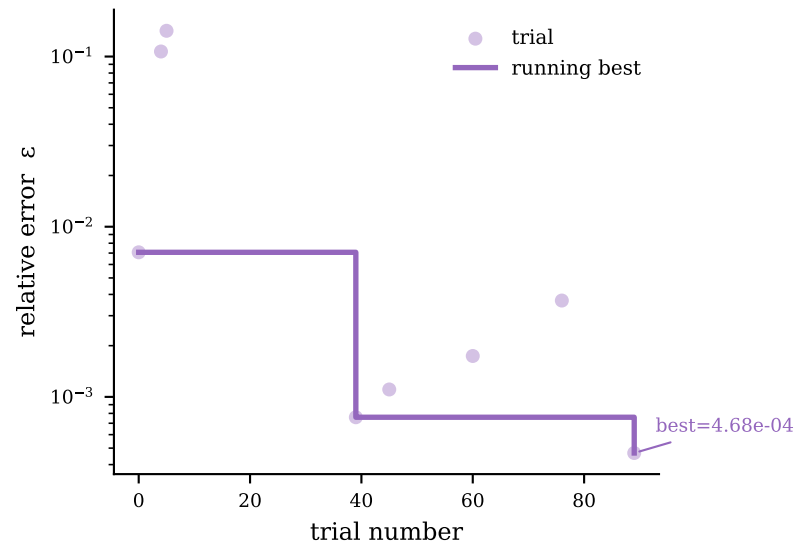
lsb (8 trials)
