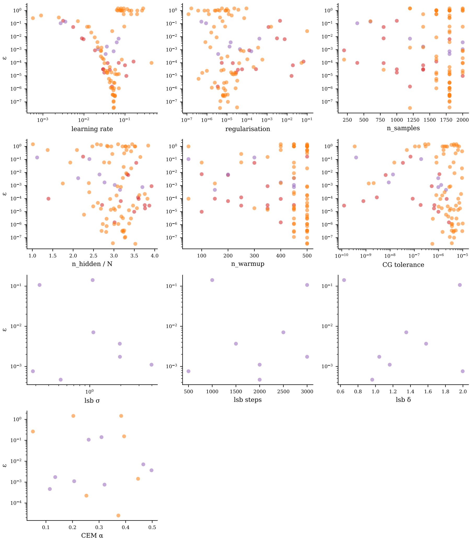
Hyperparameter sensitivity — j1j2_1d/j1j2_1d_20260527_170753/N8_J20.0
